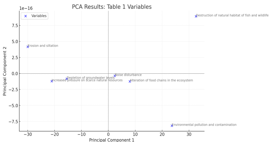
Figure 1: Principal Component Analysis Visualization of Fisheries Ecosystem Impact Variables
