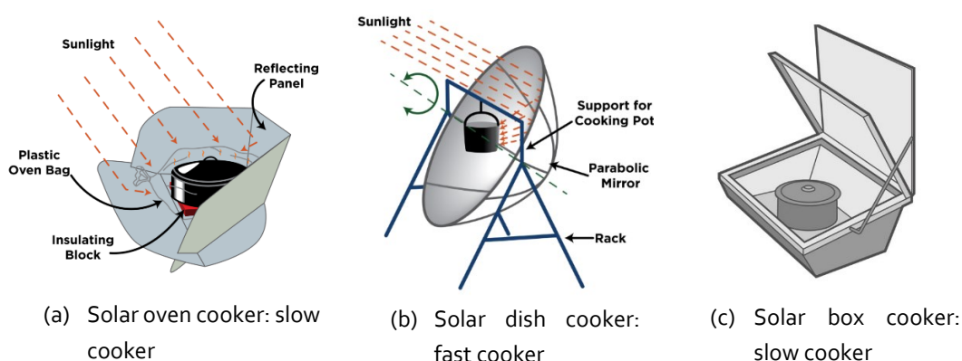
Figure 7: Different types of solar energy cookers (Gawande & Ingole, 2019)
